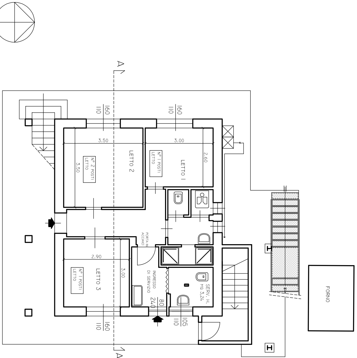
Piano terra
