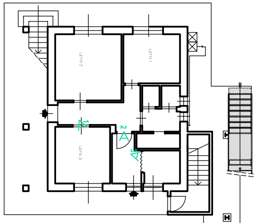
Piano terra
